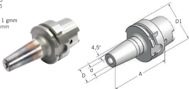
HSK - A 63
