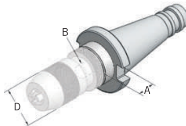
Bohrfutter / Chuck
