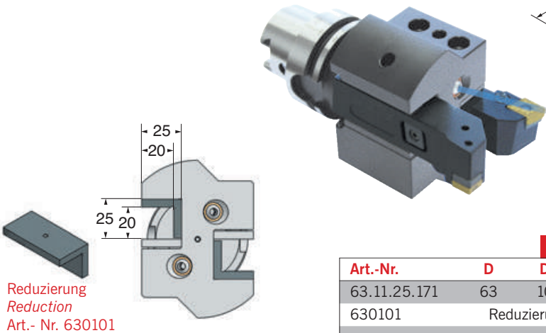
HSK - T 63
