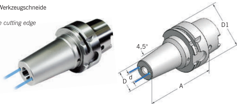
HSK - A 63
