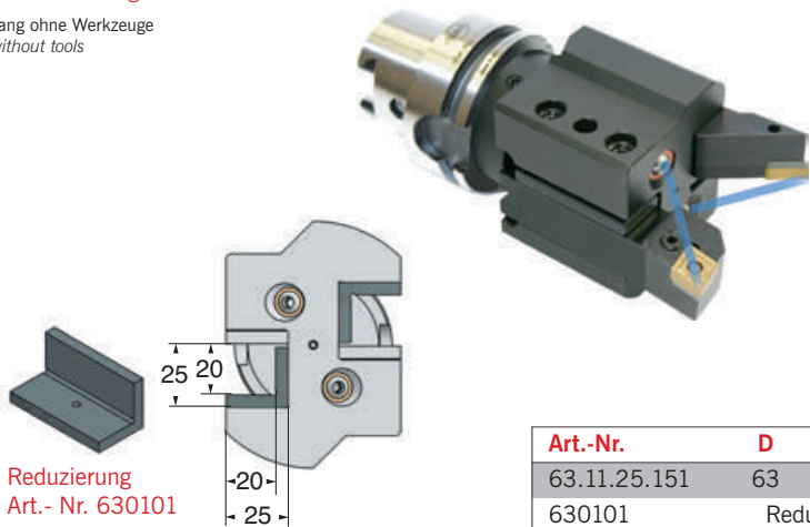
HSK - T 63
