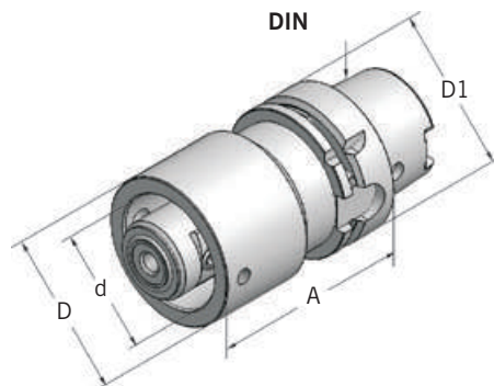
HSK - A 63
