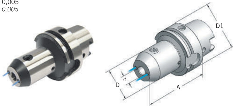
HSK - A 63
