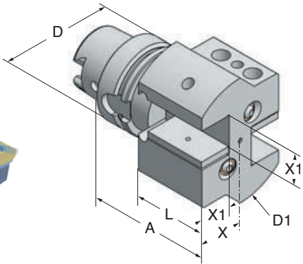
HSK - T 63
