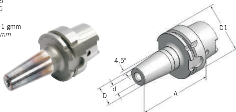
HSK - A 100
